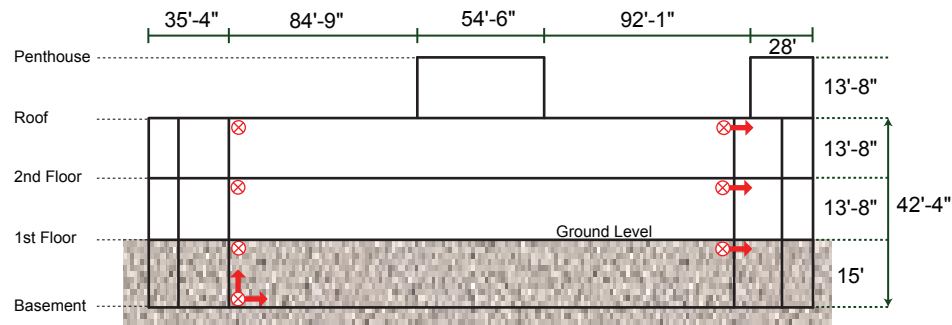
Elevation View Looking Reference North
