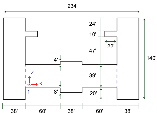
Basement
