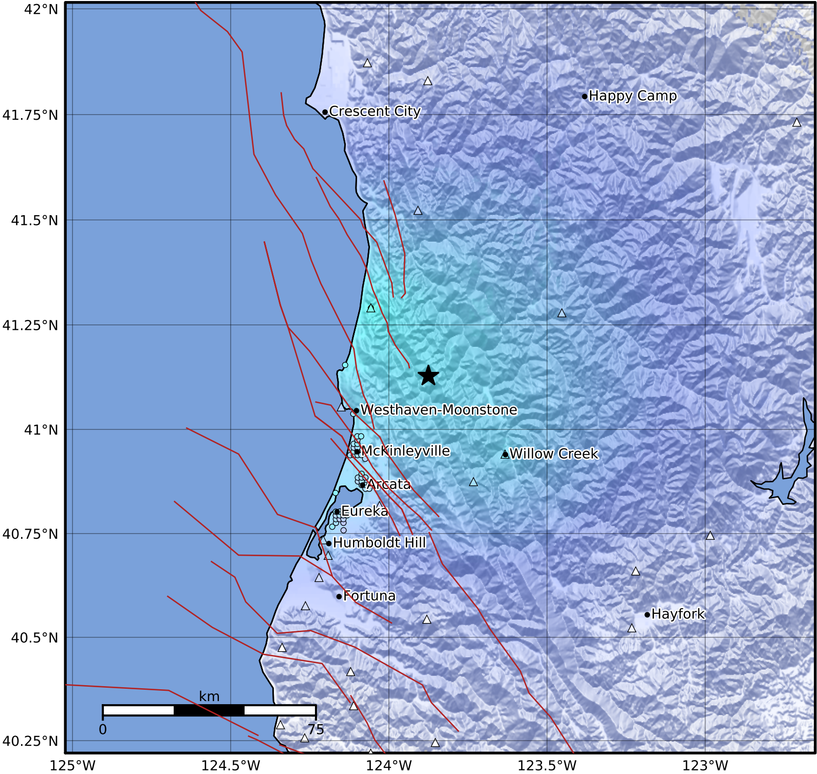
Macroseismic Intensity Map CISN/cgs ShakeMap: 16 km (10 mi) WSW of Weitchpec, CA Jan 20, 2023 08:01:14 UTC M4.3 N41.13 W123.88 Depth: 25.3km ID:73834441
